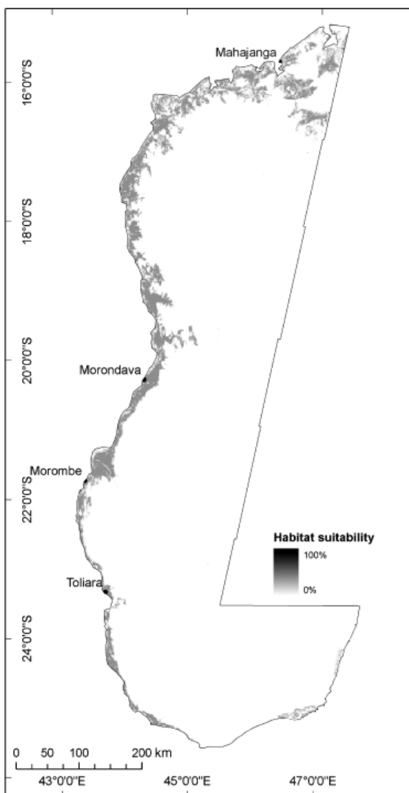
Figure 3 Final habitat suitability model.
