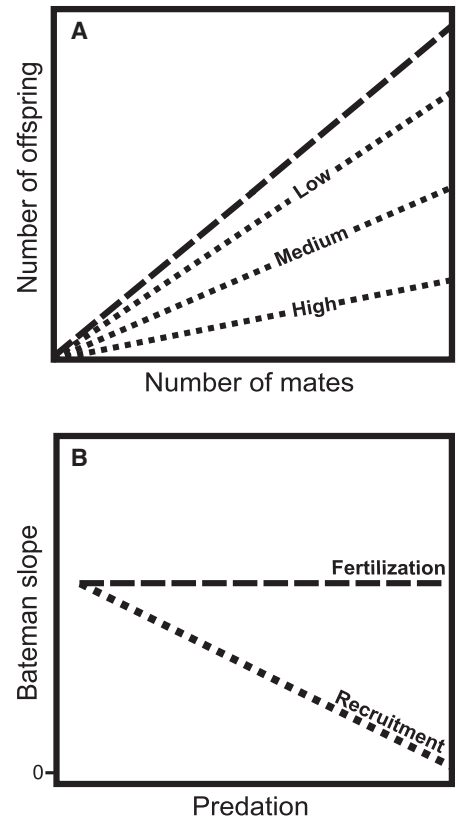
Fig. 1. Calculating the Bateman slope. The standard way of measuring the Bateman slope (usually called the “Bateman gradient”) is to regress the number of offspring at the fertilization stage (dashed line) onto mating success (A). The method used by Byers and Dunn is instead to measure reproductive success at the later, recruitment stage (dotted lines), where the difference between the dashed and dotted lines can be interpreted as fawn mortality. In this illustration, different levels of predation affect the number of offspring measured at the recruitment stage but do not affect the number of offspring at the fertilization stage. The consequences of this for the calculated Bateman slopes are shown in (B), where predation does not affect the Bateman slope under the standard definition but necessarily does affect the metric employed by Byers and Dunn. We agree that the dotted line represents a biologically relevant scenario but suggest that it should not be confused with, and needs to be distinguished from, the dashed line. We suggest that a new term, such as “effective Bateman slope” (or “effective Bateman gradient”), may be more appropriate when researchers measure a Bateman slope in terms of surviving offspring.
